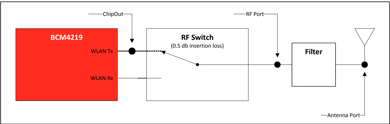
Figure 20: RF Port Location
