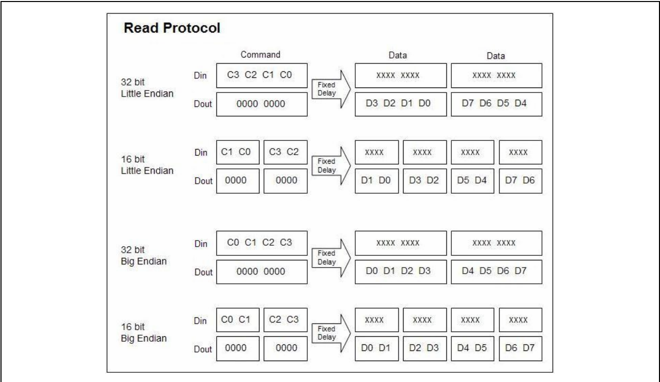
Figure 10: SPI Read Protocol
