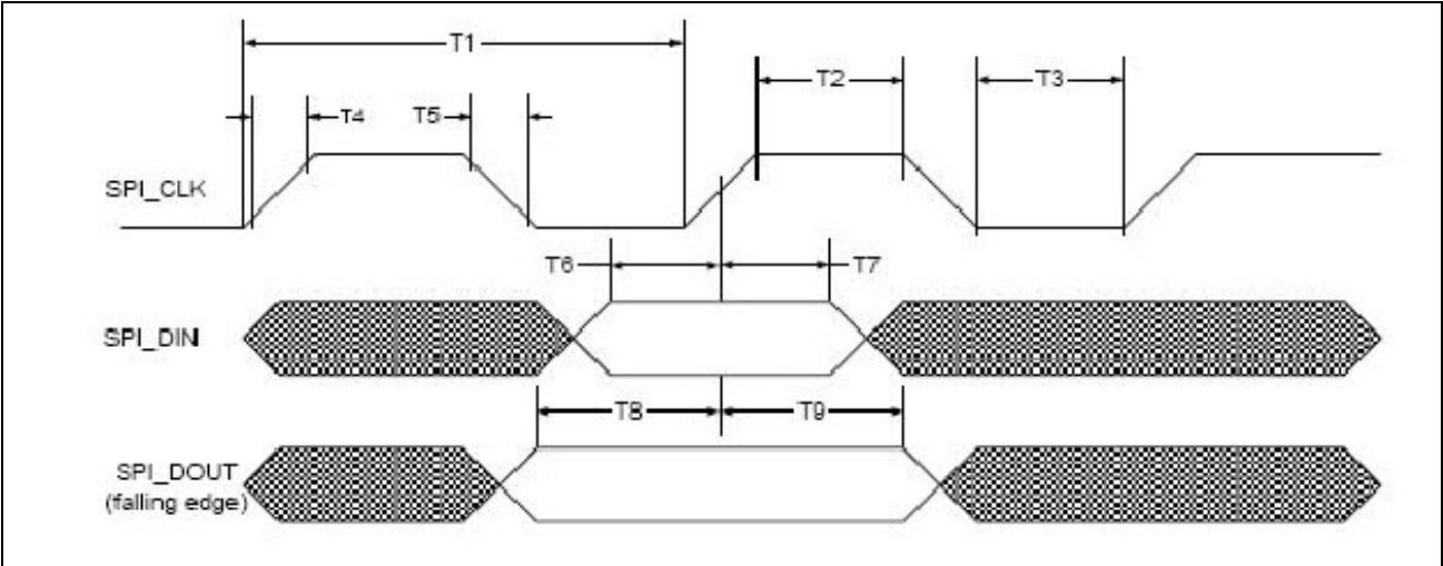
Figure 22: gSPI Timing
